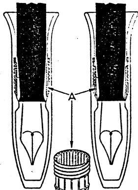
TURNING PEN TO THE RIGHT FORCES FLUTED SLEEVE "A" INTO LOCKING POSITION MAKING AIR-TIGHT SEAL BY FIRMLY PRESSING PEN AGAINST SOCKET SEAT
